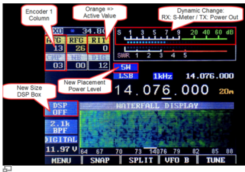
UHSDR Basic Screen Layout (from Github UHSDR)
